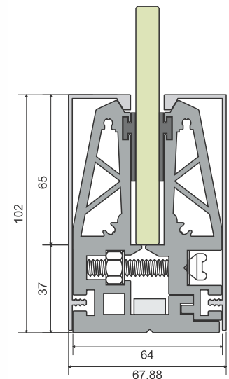
ALRL-01 (S)
